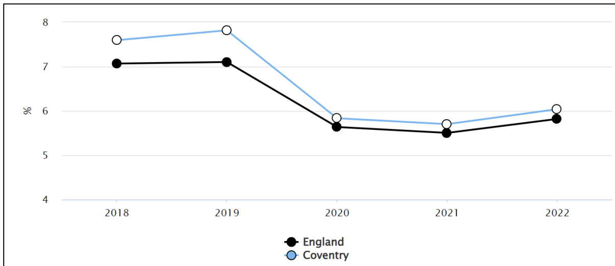
Figure 2.1 – Fraction of mortality attributable to particulate air pollution (new method) for Coventry and England.
