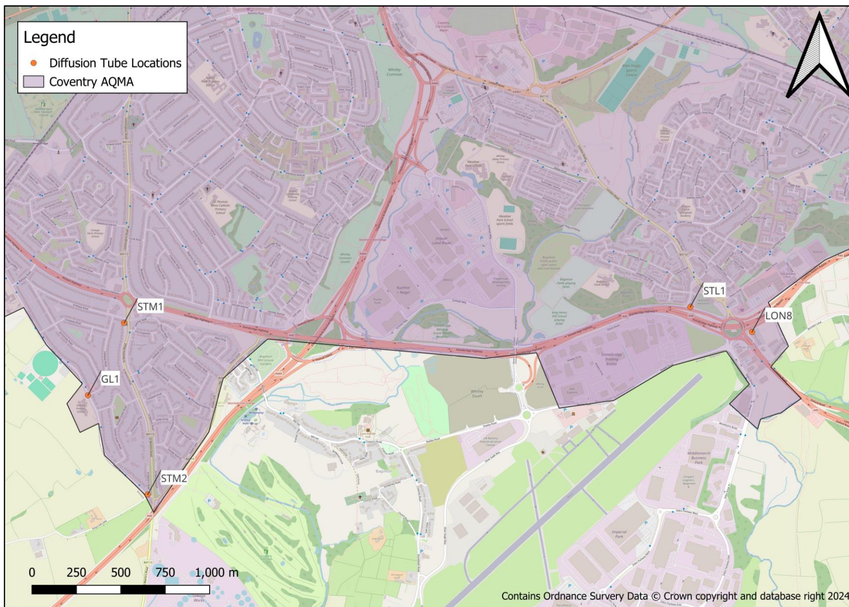
Figure D.9 – Maps of Diffusion tubes across Coventry (Stonebridge Highway)
